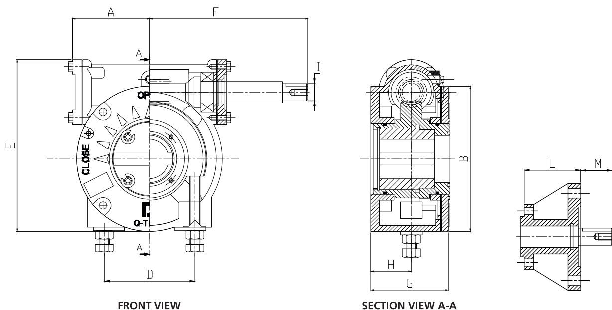
FIG (1) – Standard Gear Box
