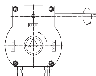
Right Hand Anti-Clockwise to Open from Close
