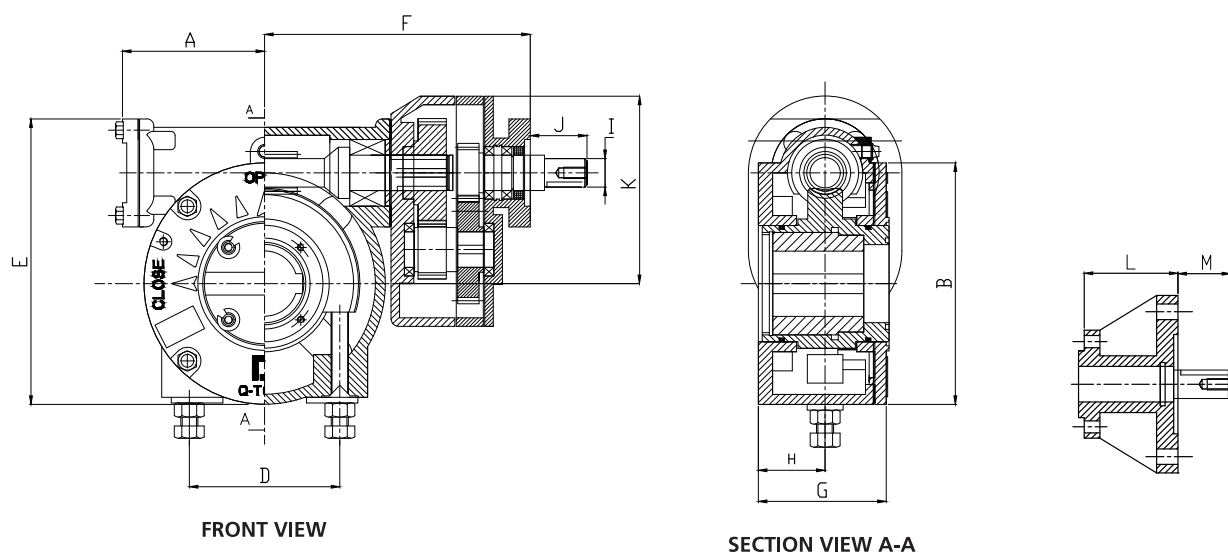
■ FIG (3) – Standard Gear Box with Double Reduction Unit
