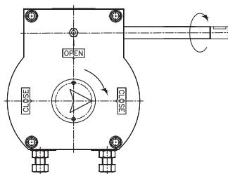
Right Hand (Standard Supply) Clockwise to Close from Open
