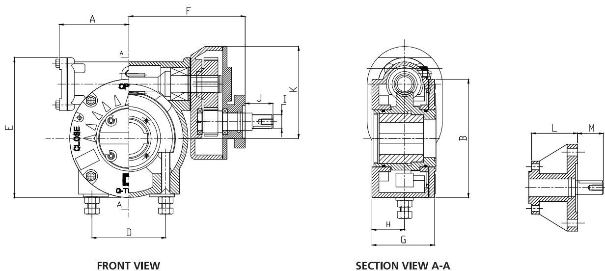
■ FIG (2) – Standard Gear Box with Single Reduction Unit
