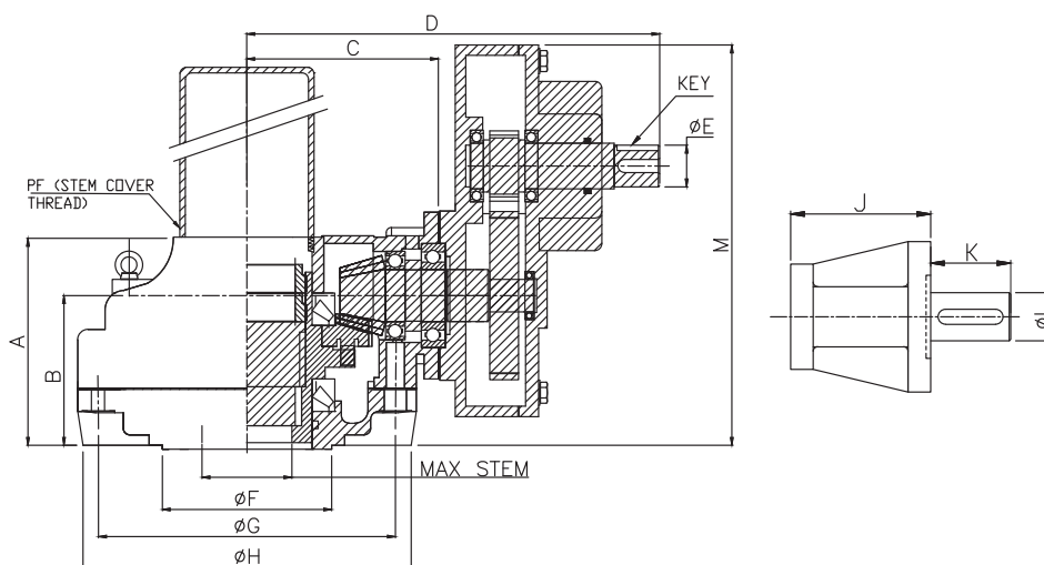
■ FIG(2)-Standard Gear Box with Single Reduction Unit
