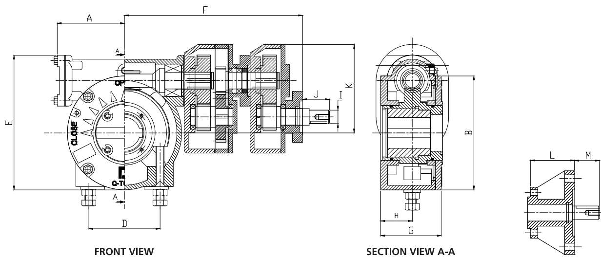
■ FIG (4) – Standard Gear Box with Triple Reduction Unit
